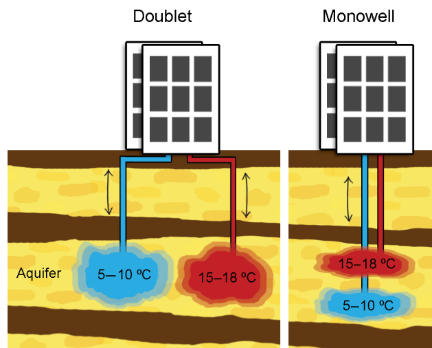
Figure 2. Schematic representation of ATEs doublet and monowell.
